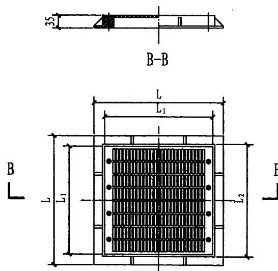
WL-ADP336回水口
