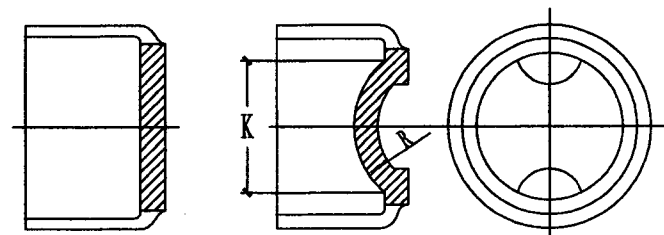
DN ≤ 300 插堵
