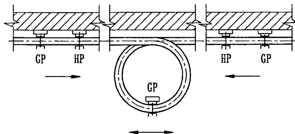
环形补偿
