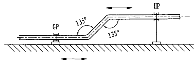
Z形补偿
