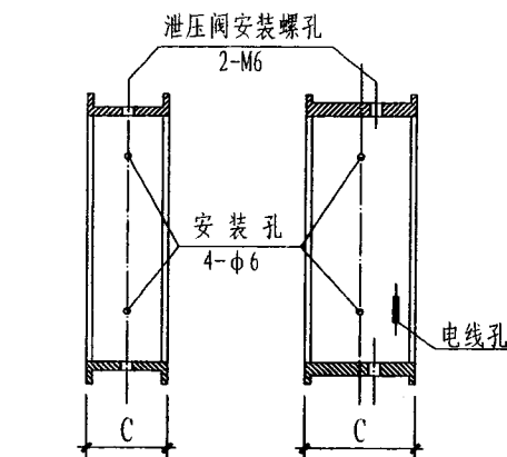
FXY-I (II) WKZX-013 (025)型左视图 FXY-I (III)型左视图
