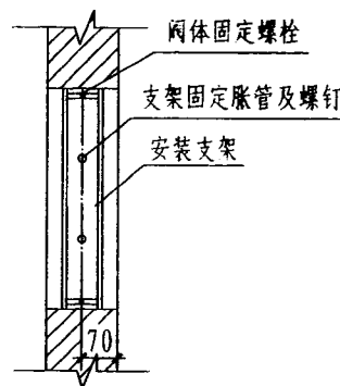
FXY-I (II) WKZX-013 (025) 型泄压阀支架安装图
