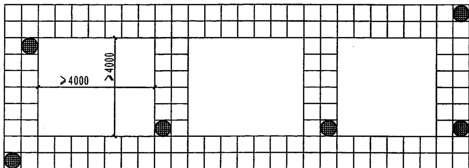
(2) 梯形布置
