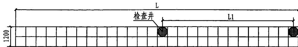
(1) 沟型布置
