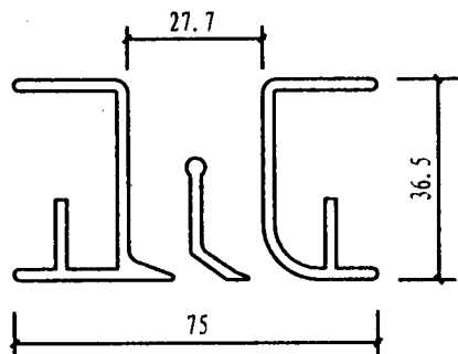
XS (单向气流型)
