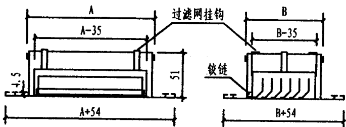
MJ (铝质细叶片)
