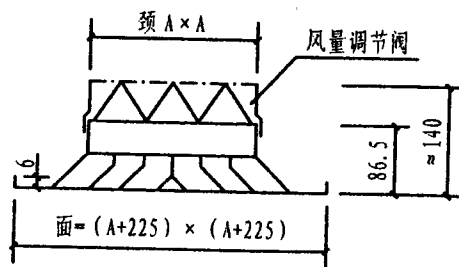
FS (钢)
