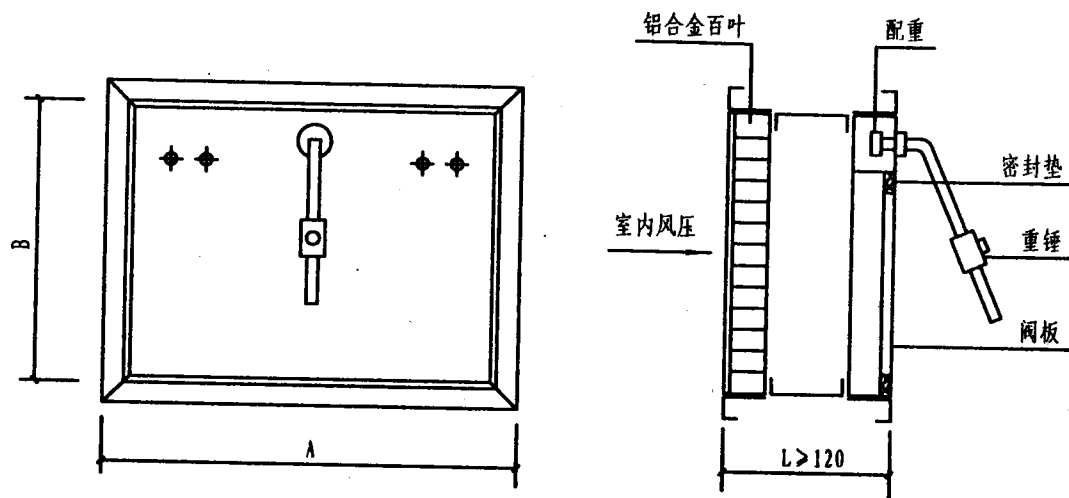
HA余压阀
