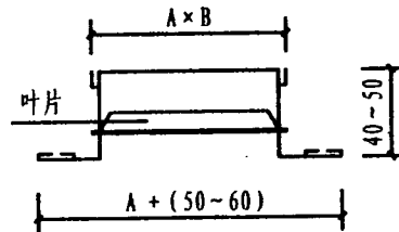
DB (单层百叶)
