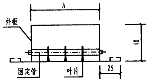
TF (直片型)
